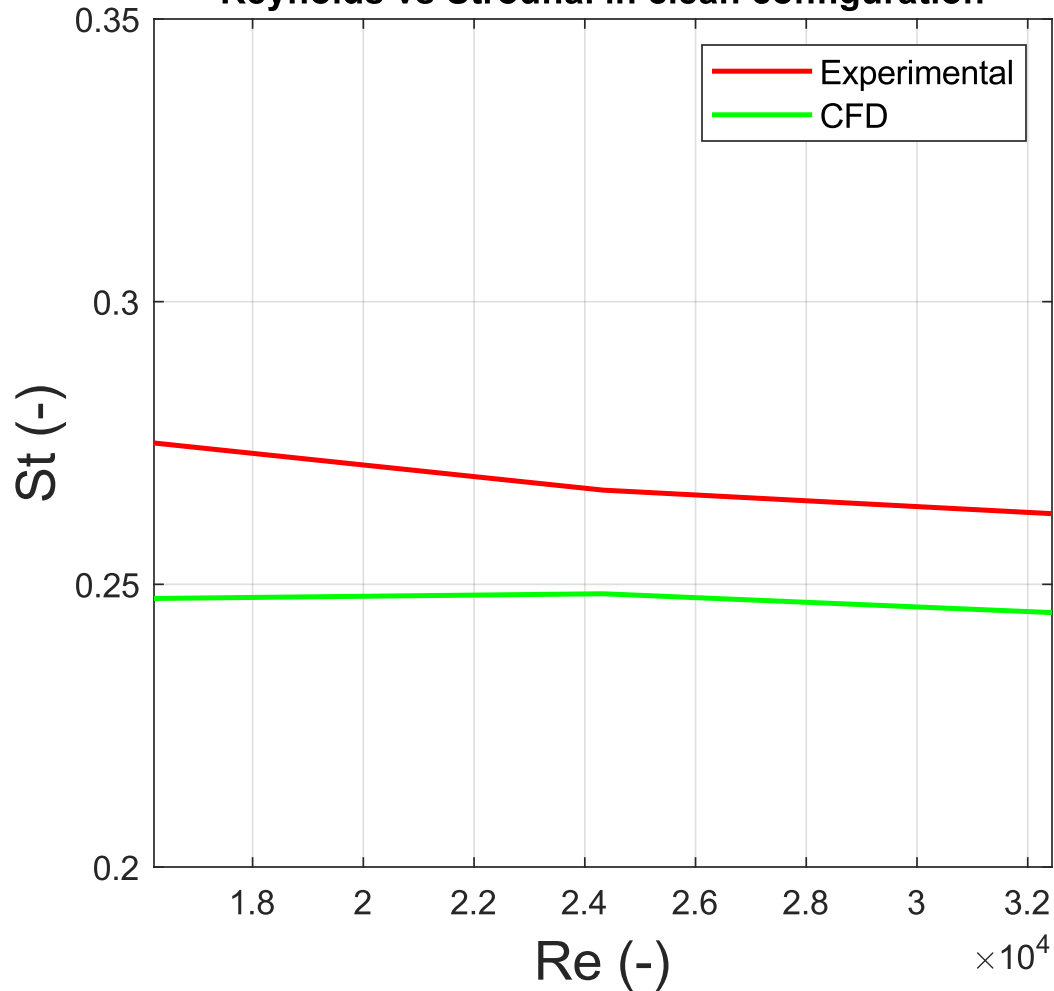
Reynolds vs Strouhal in clean configuration
